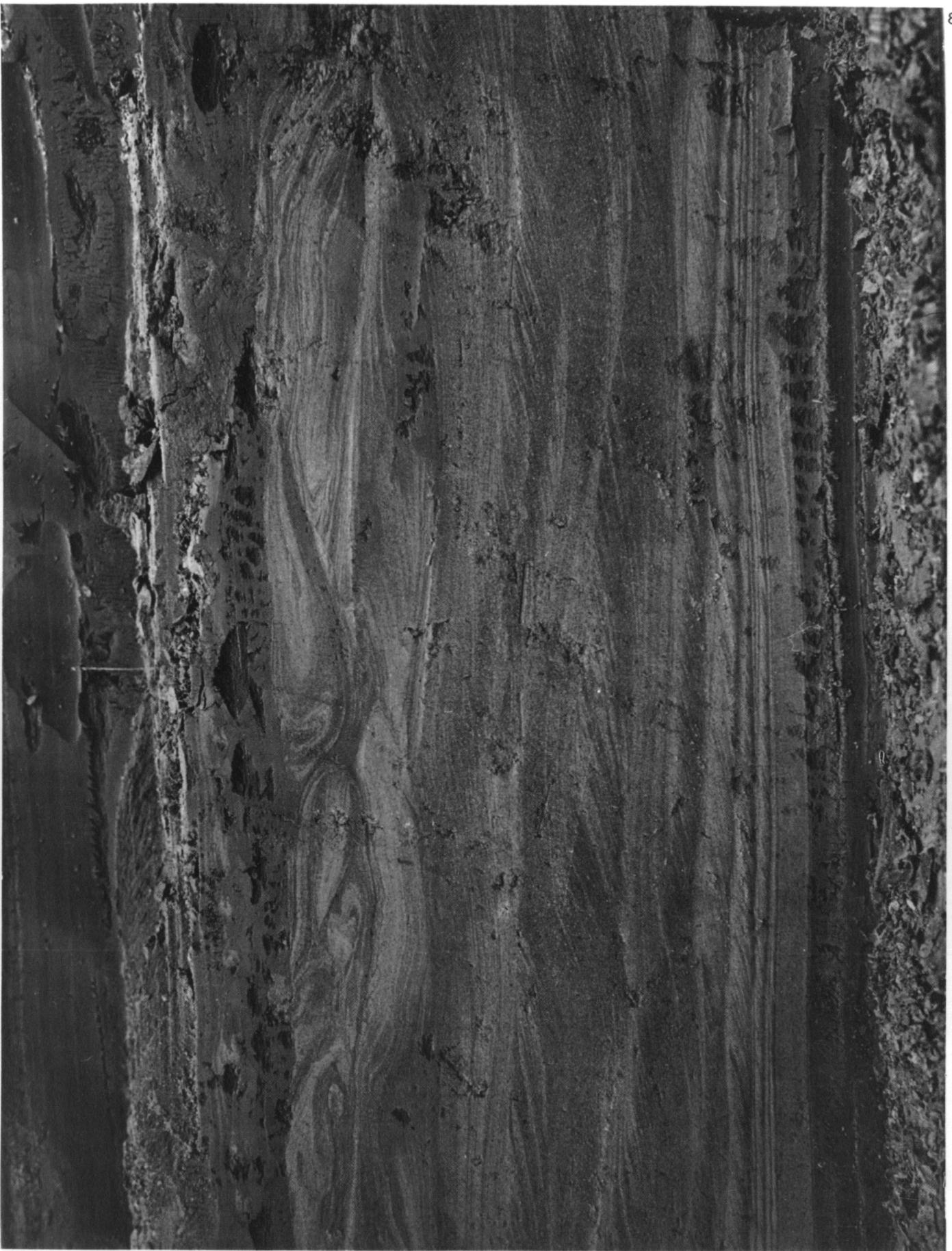
Figure 5 A 26 cm sand bed near the base of the section at Combe de la Poya. Ripple-drift cross-lamination indicates current from the right with truncation of laminae on the stoss side. The top of the unit has been deformed by penecontemporaneous slumping.
